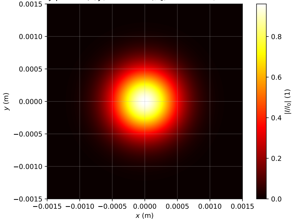
Intensity profile I(x, y, z = 0.637m)/I_0 , Pin=0.2Pcr, artificial time
